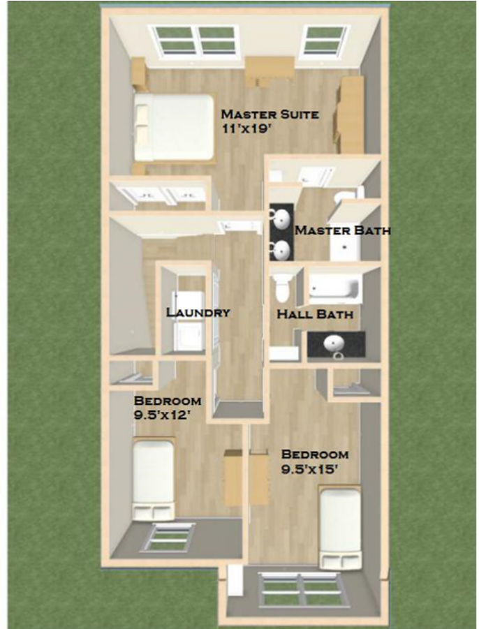
SECOND FLOOR LAYOUT
