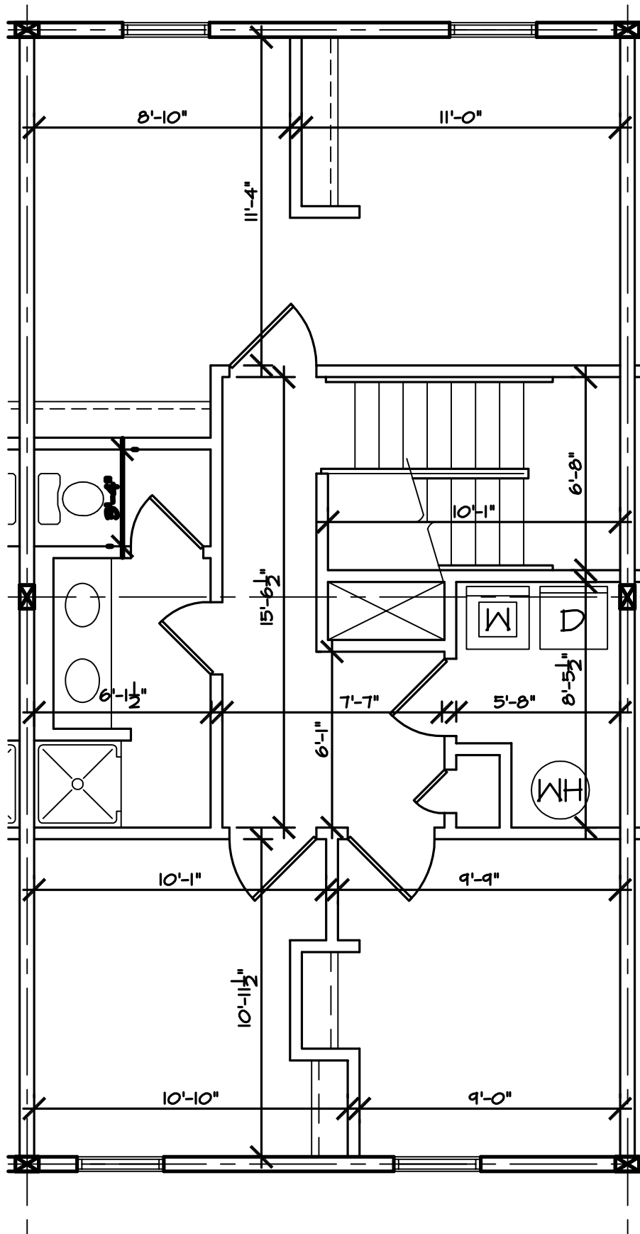
1 UNIT TYPE A (2ND FLR) A-2 SCALE: 1/8" = 1'-0"
