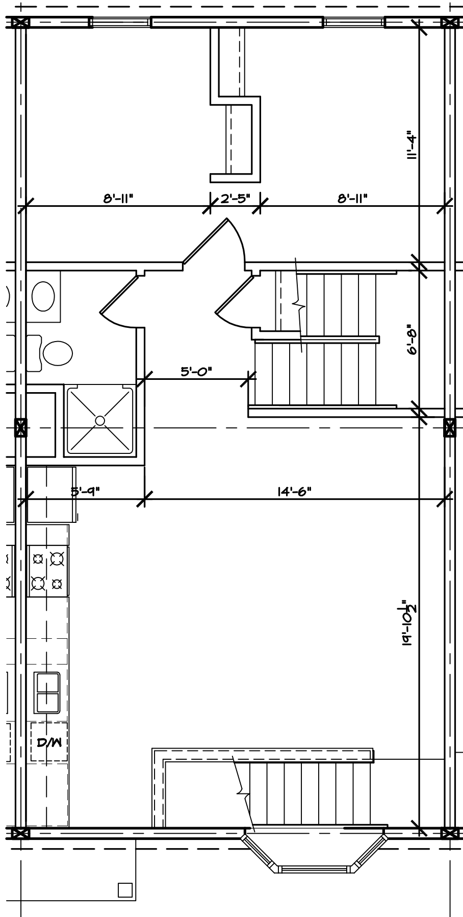
1 A-2 UNIT TYPE A (1ST FLR) SCALE: 1/8" = 1'-0"
