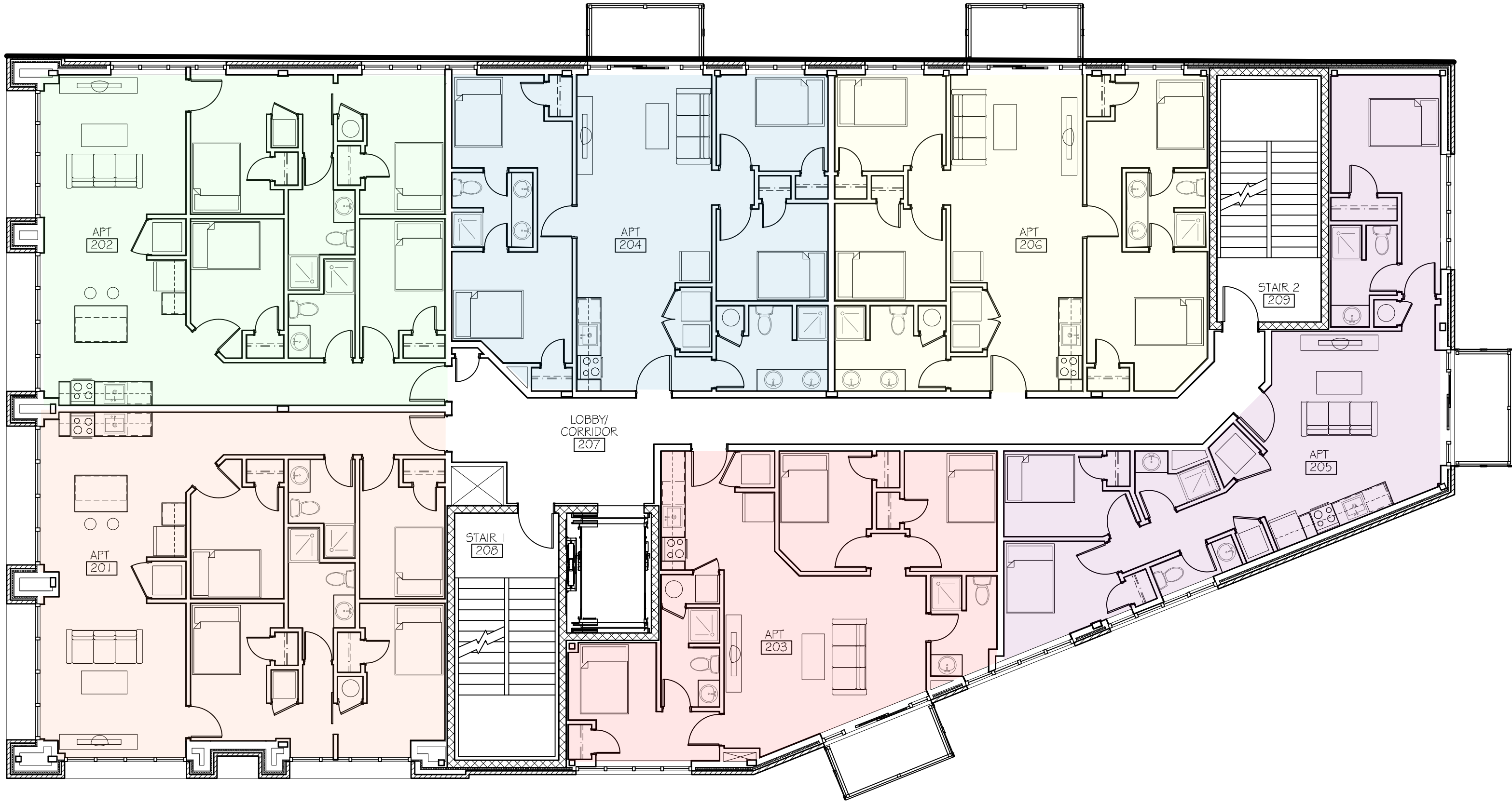
1 SECOND FLOOR APARTMENT PLAN SCALE: 1/4" = 1'-0"
